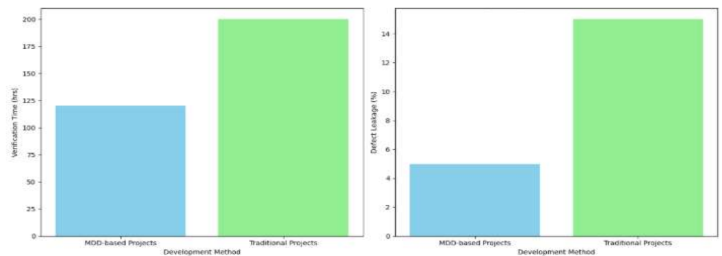
Figure 2. Verification Time Reduction in MDD vs. Traditional Methods, Defect Leakage Comparison in MDD vs. Traditional Methods.
