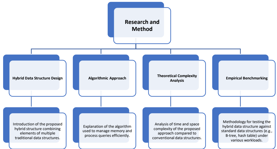
Figure 1. Flowchart structure.
