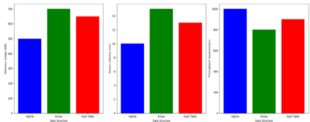
Figure 2,3,4 Memory Usage Comparison, Query Latency Comparison, Throughput Comparison.
