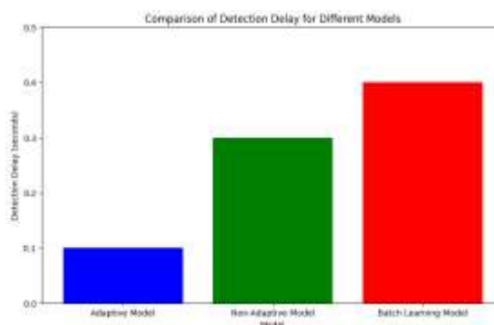
Figure 3. Comparison of Detection Delay for Different Models.
