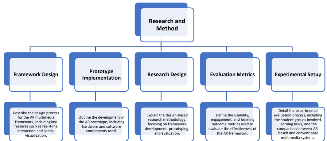
Figure 1. Flowchart structure.
